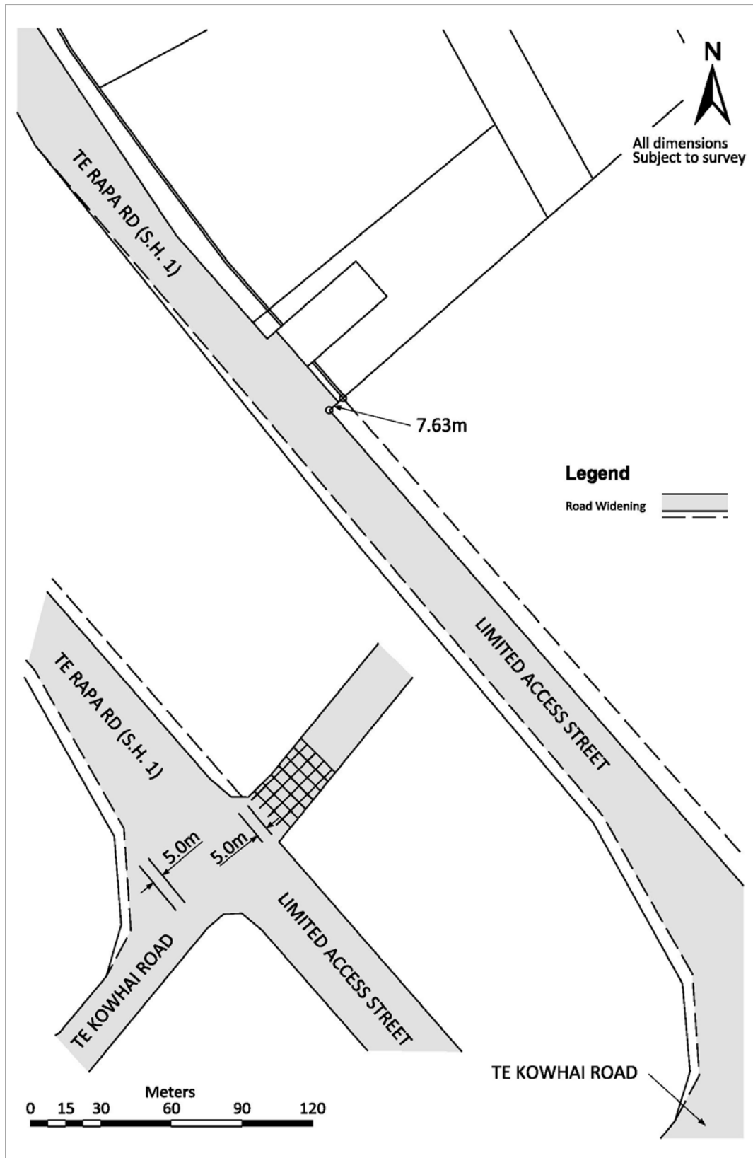
Figure 16-3: Designation E87 – Road Widening (Te Rapa Road/Te Kowhai Road)
