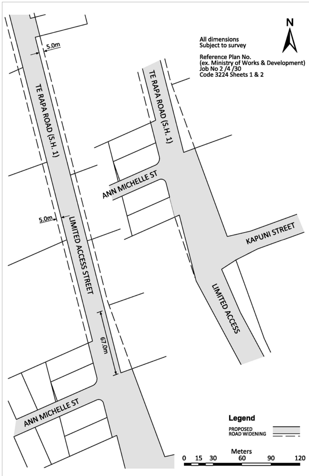
Figure 16-2: Designation E86 – Proposed Road Widening (Te Rapa Road/Ann Michelle Street)
