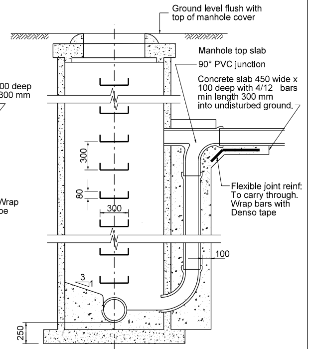
DROP MANHOLES WITH EXTERNAL DROP PRE-CAST BASE (Sanitary Sewer Only)
